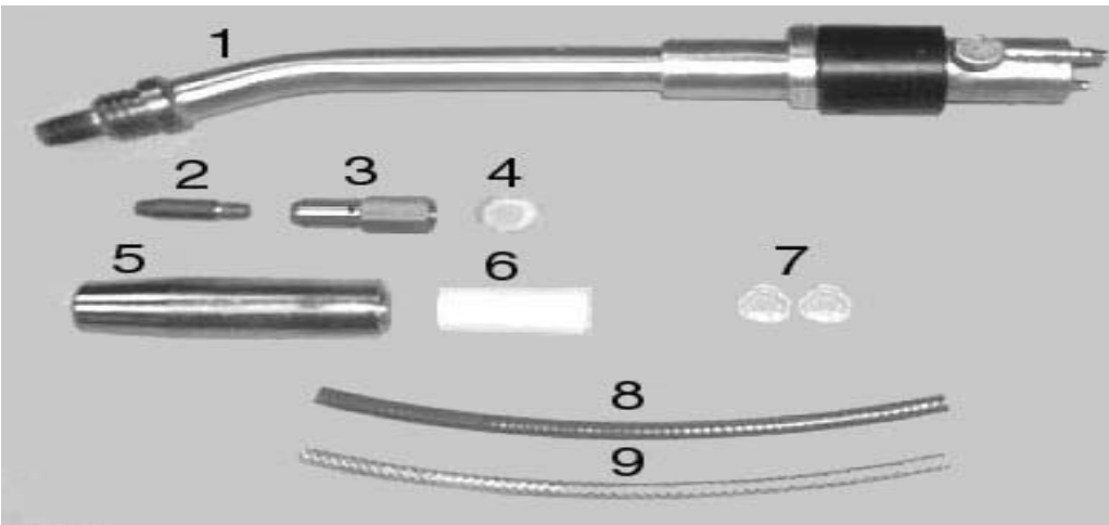
Extended T.C.P. 22° Robotic Neck Assembly (PARTS BREAKDOWN)
