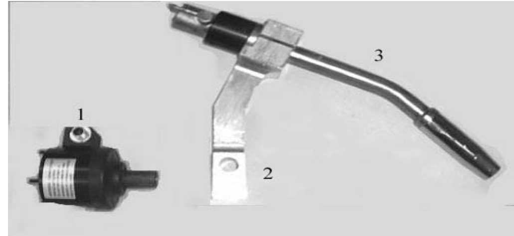
Extended T.C.P. 23° Bracket / 22° Torch (PARTS BREAKDOWN)
