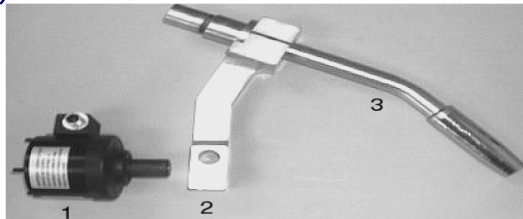
Standard T.C.P. 23° Bracket / 22° Torch (PARTS BREAKDOWN)
