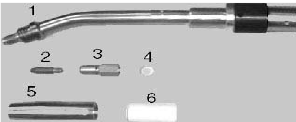
Standard T.C.P. 22° Robotic Neck Assembly (PARTS BREAKDOWN)
