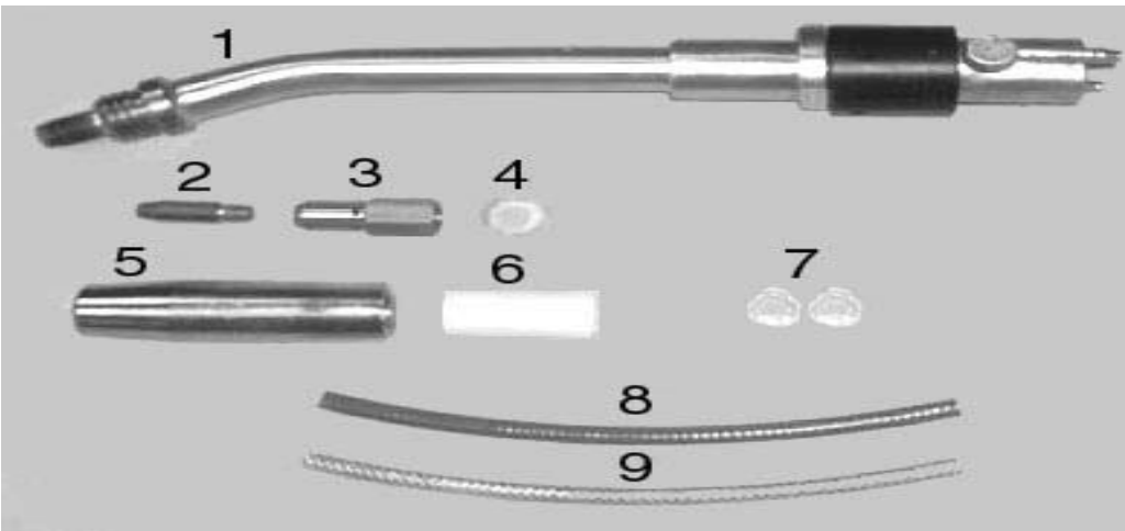
Standard T.C.P. 22° Robotic Neck Assembly (PARTS BREAKDOWN)
