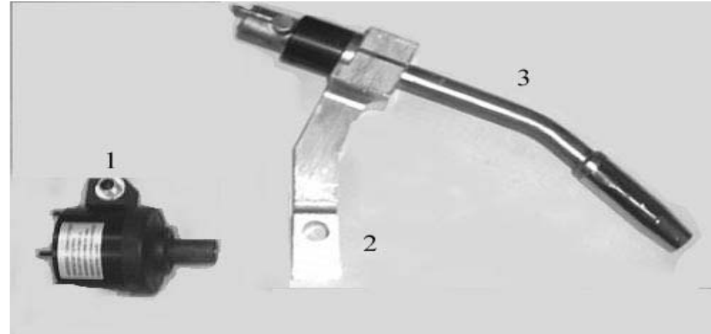
Standard T.C.P. 23° Bracket / 22° Torch (PARTS BREAKDOWN)
