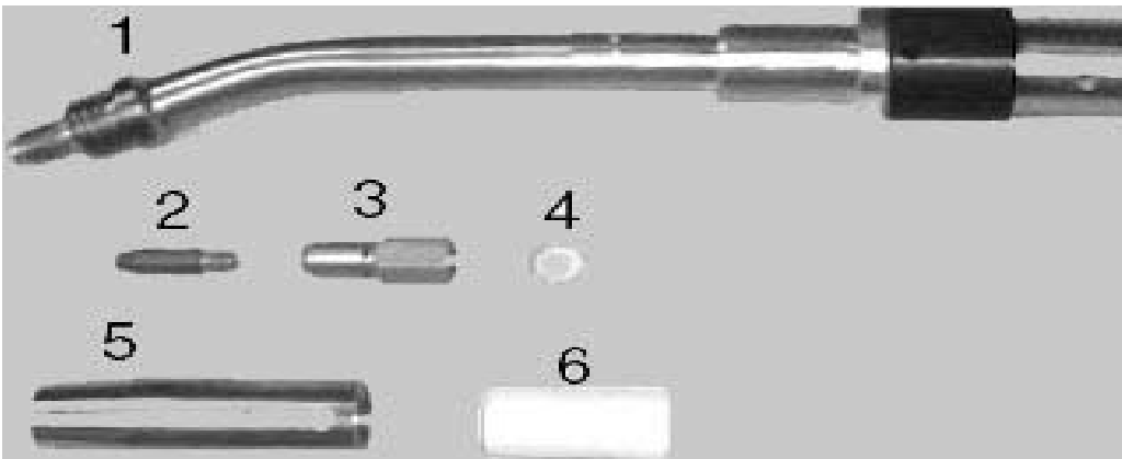
Extended T.C.P. 22° Robotic Neck Assembly (PARTS BREAKDOWN)
