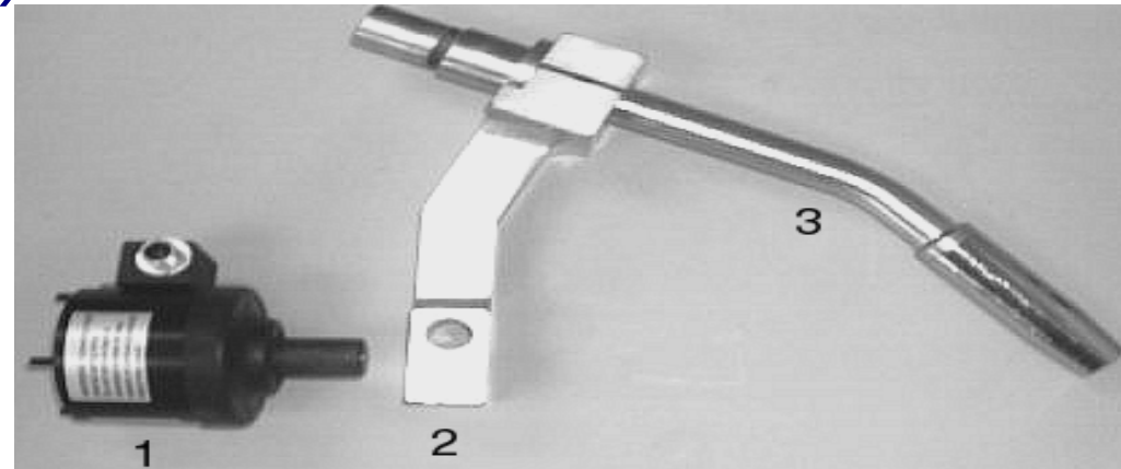
Extended T.C.P. 23° Bracket / 22° Torch (PARTS BREAKDOWN)
