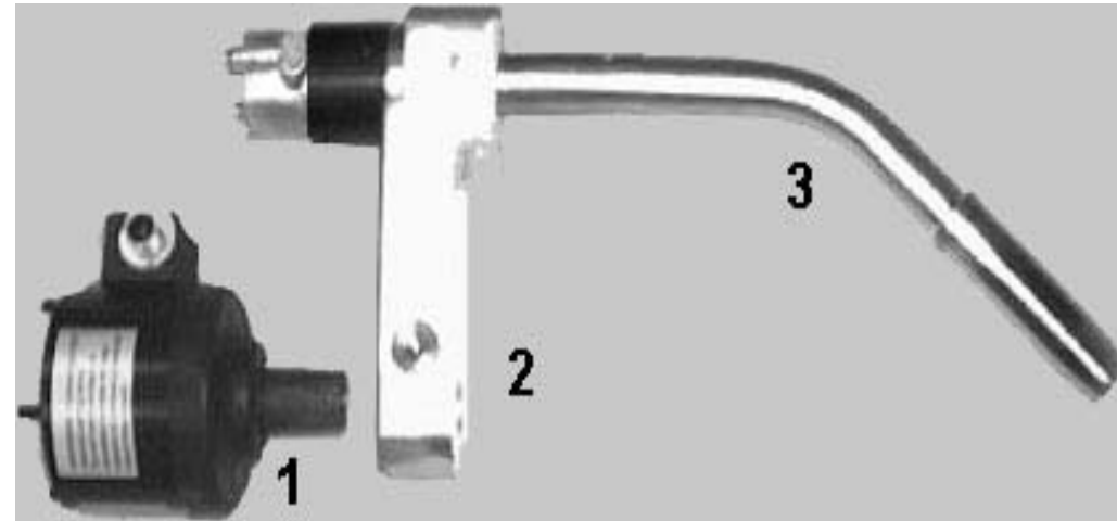
Extended T.C.P. 180° Bracket / 45° Torch (PARTS BREAKDOWN)
