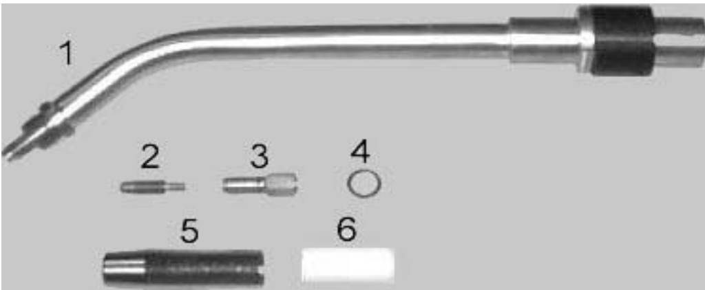
Standard T.C.P. 45° Robotic Neck Assembly (PARTS BREAKDOWN)
