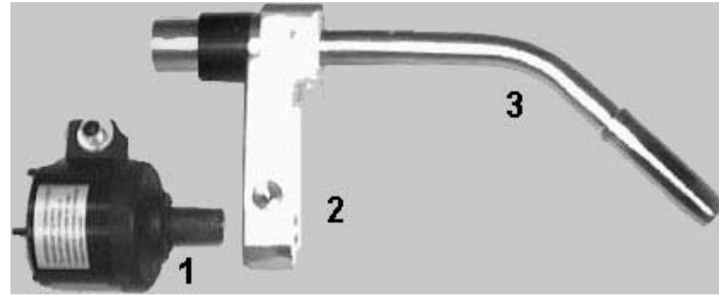
Standard T.C.P. 180° Bracket / 45° Torch (PARTS BREAKDOWN)
