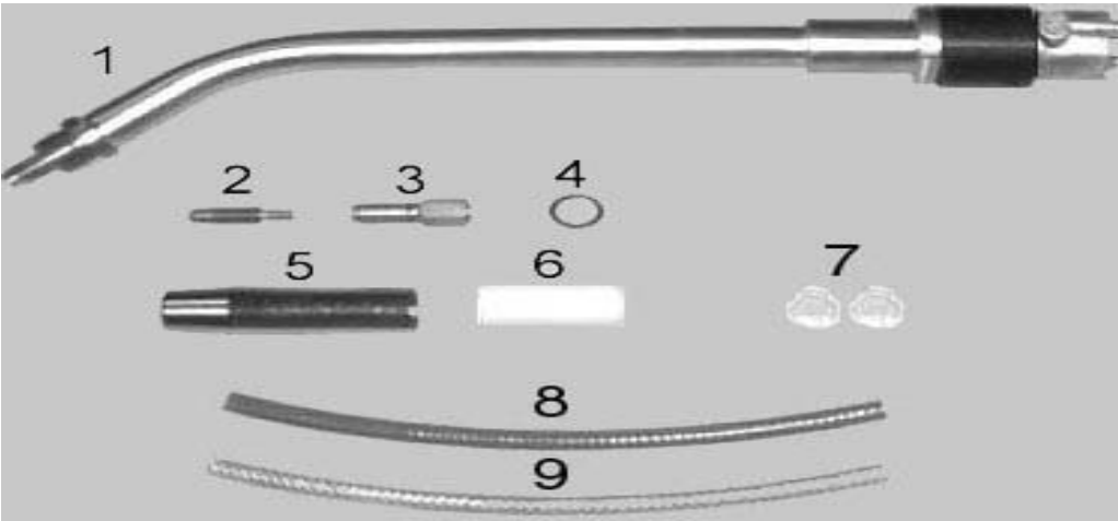
Standard T.C.P. 45° Robotic Neck Assembly (PARTS BREAKDOWN)
