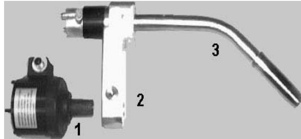
Standard T.C.P. 180° Bracket / 45° Torch (PARTS BREAKDOWN)
